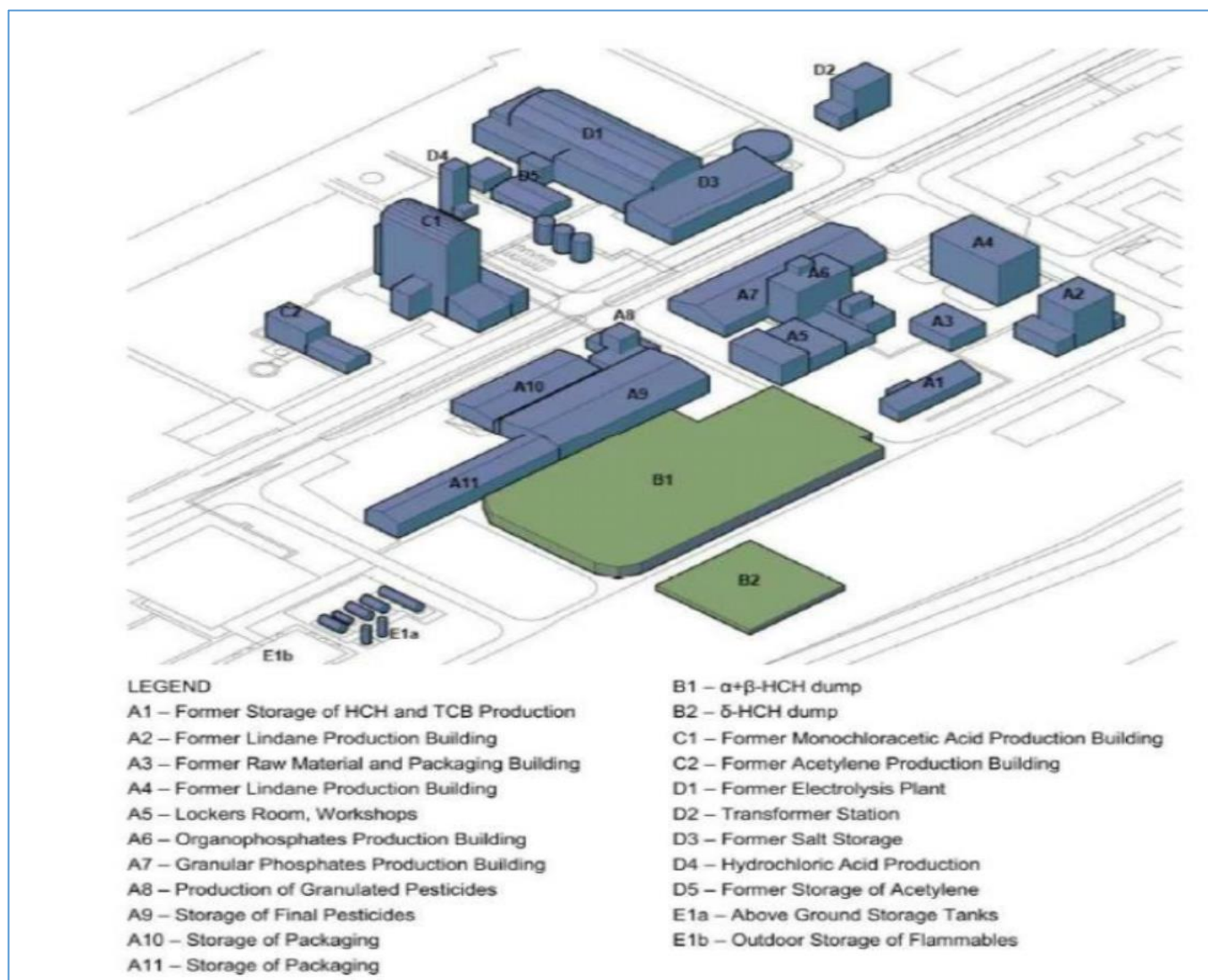
Figure 1: Illustration of the OHIS plant layout (source Polyeco)
